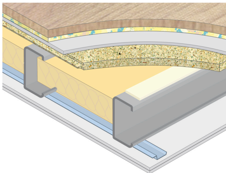
Monarfloor® Deck 22 Decorative on a timber sub-floor supported by steel joists.
