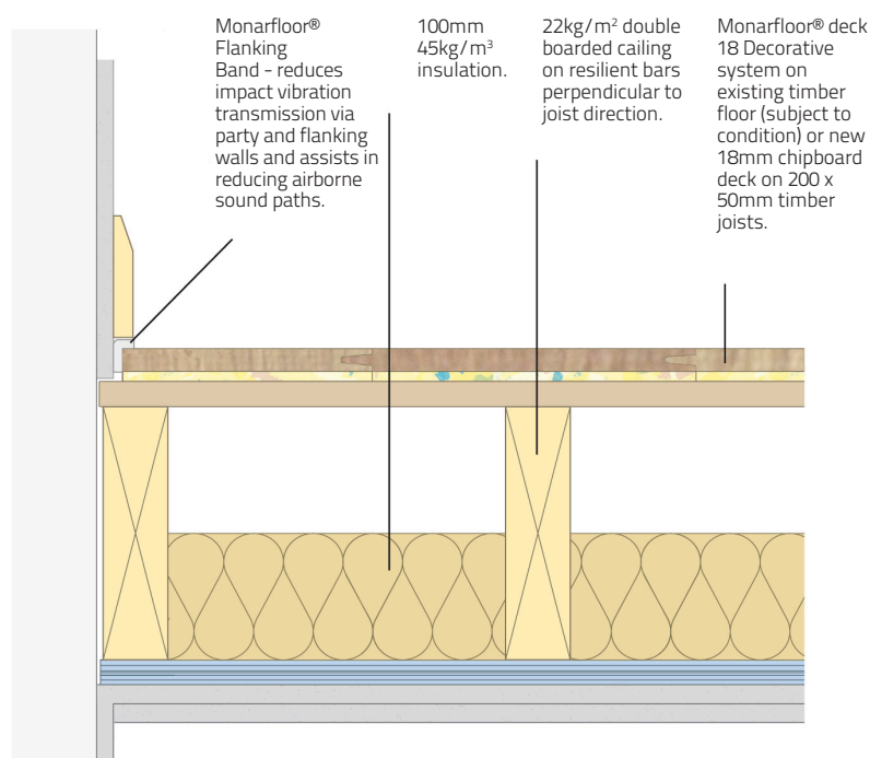
Monarfloor® Deck 22 Decorative on a timber floor with a resilient bar system.
