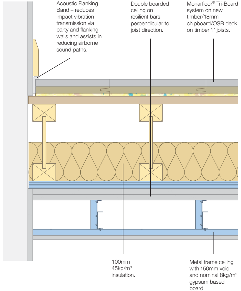
Monarfloor® Tri-Board System on a timber sub-floor with a resilient bar and metal frame ceiling.
