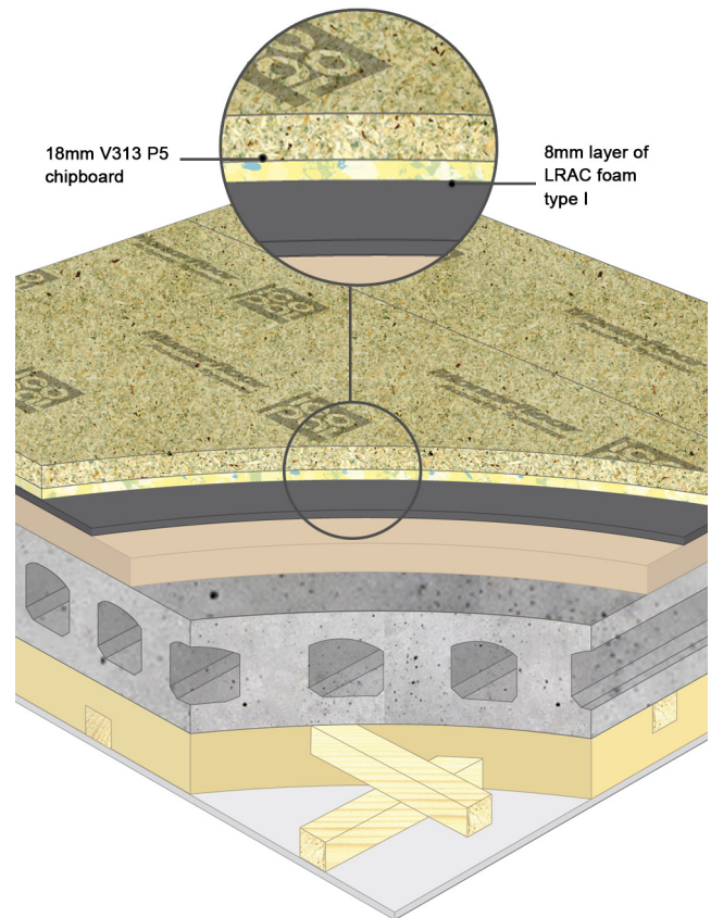
Monarfloor® Impact 18 on a concrete deck.
