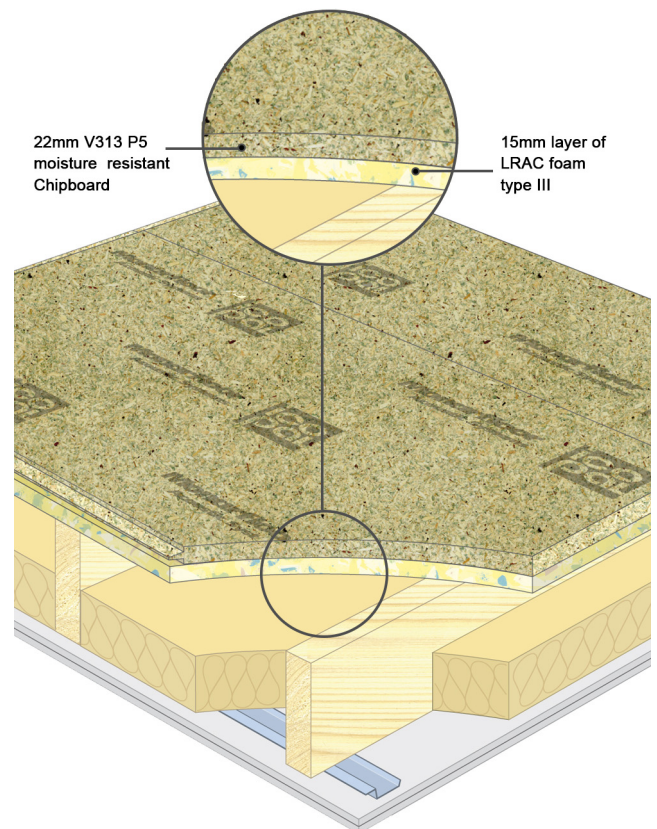
Monarfloor® Structure Deck on a timber joists
